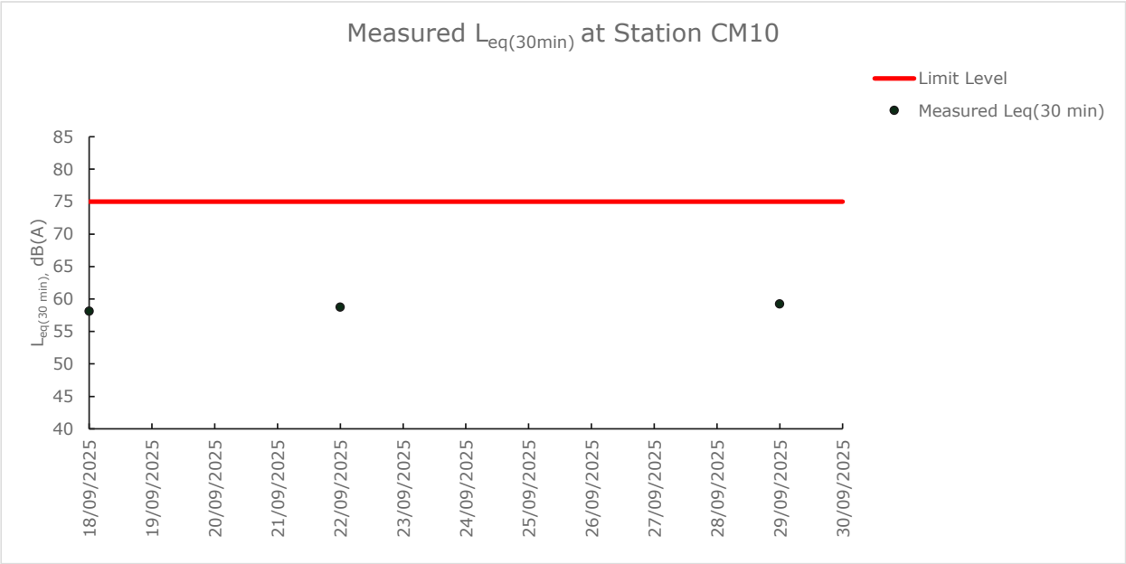
Graphical Presentation For Noise Monitoring at Station CM10 (for Works Contract No. ND/2024/10)
